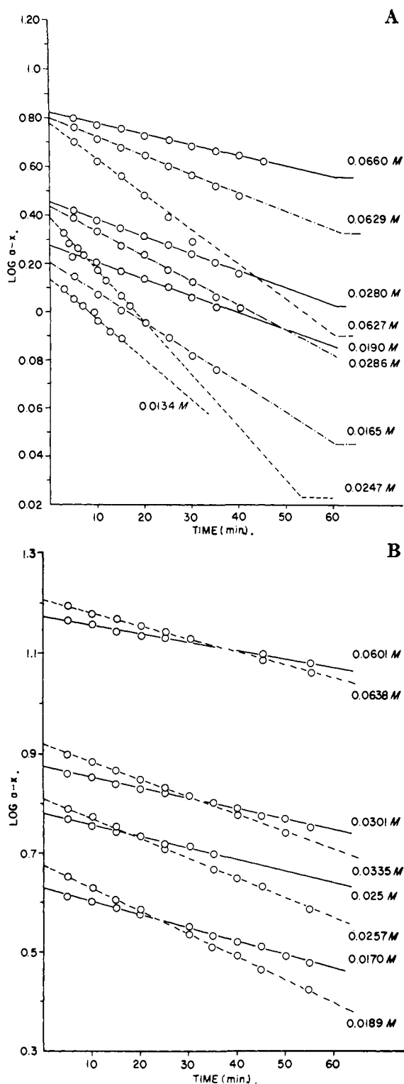
Fig. 2.—Estimation of initial velocities from apparent first-order plots; [S]_0 (initial concn.) ethyl 5-( p -hydroxyphenyl)-3-ketovaleate: (A) a - x = \text{ml.} \times 10 of 0.5 N NaOH per 5 ml. of digest; —, E = 0.5 mg. of N/ml.; — — —, 1 mg. of protein N/ml.; - - - -, 2 mg. of protein N/ml. (B) a - x = \text{ml.} \times 10 of 0.2 N NaOH per 5 ml. of digest; 0.02 M tris-(hydroxymethyl)-aminomethane-HCl buffer at 25° and pH 7.9: —, E = 1/8 mg. of protein N/ml.; - - - -, 1/4 mg. of protein N/ml.
