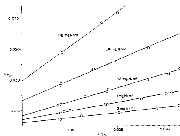
Fig. 3.— \alpha -Chymotrypsin-catalyzed hydrolysis of ethyl 5-( p -hydroxyphenyl)-3-ketovaleate at 25° and pH 7.9; v_0 in units of 10^{-6} M /min.; 0.02 M tris-(hydroxymethyl)-aminomethane-HCl.
