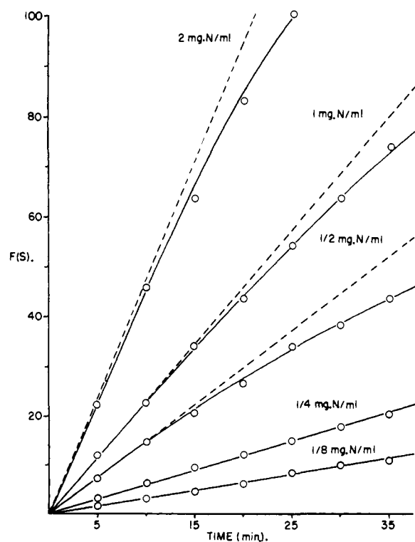
Fig. 4.—Plot of F(S) = K_s \ln [S]_0/[S] + ([S]_0 - [S]) in units of 10^3 M versus time for \alpha -chymotrypsin and ethyl 5-( p -hydroxyphenyl)-3-ketovaleate at 25° and pH 7.9; [S]_0 = 60 \times 10^{-3} M .
